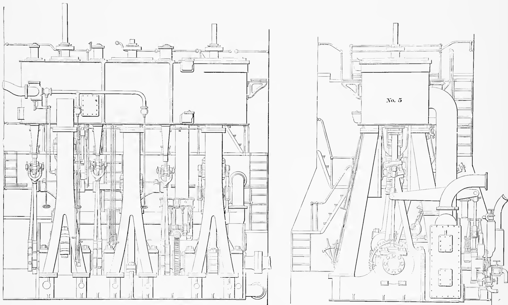
TRIPLE-EXPANSION ENGINE OF NEW STEAMSHIP HOWARD, OF THE MERCHANTS' & MINERS' LINE, BALTIMORE, MD.
